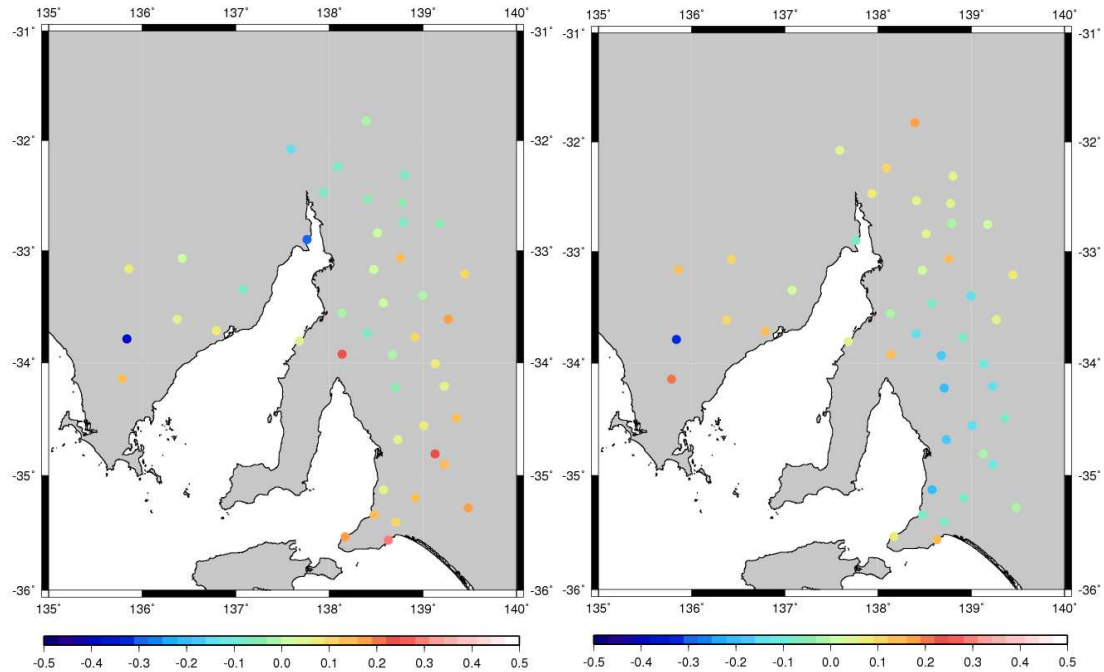
Fig 25. Differences between height anomalies from GPS-leveilling observations and AUSGeoid98 (left) and EGM2008 (right) over the SASZ [Mercator projection; units in metres]
