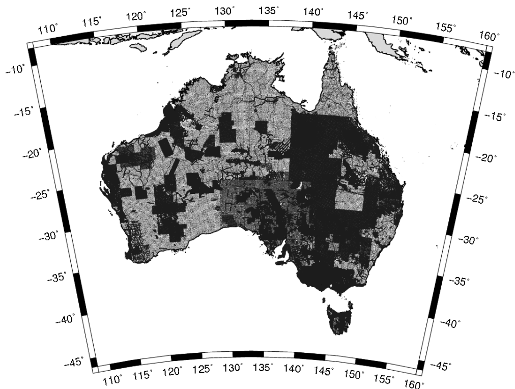
Fig 2. Coverage of the 1,304,904 Australian land gravity observations in the June 2008 data release from Geoscience Australia (Lambert projection)
