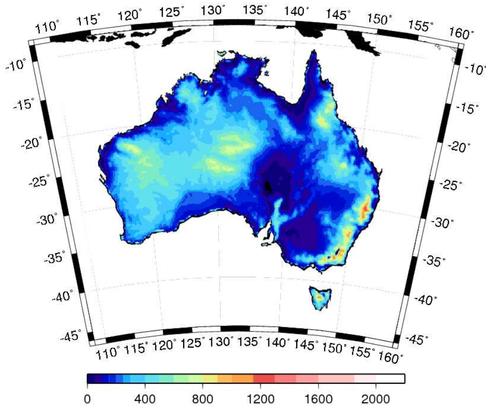
Fig 12. Australian topography from the version 2.1 DEM [Lambert projection; units in metres]
