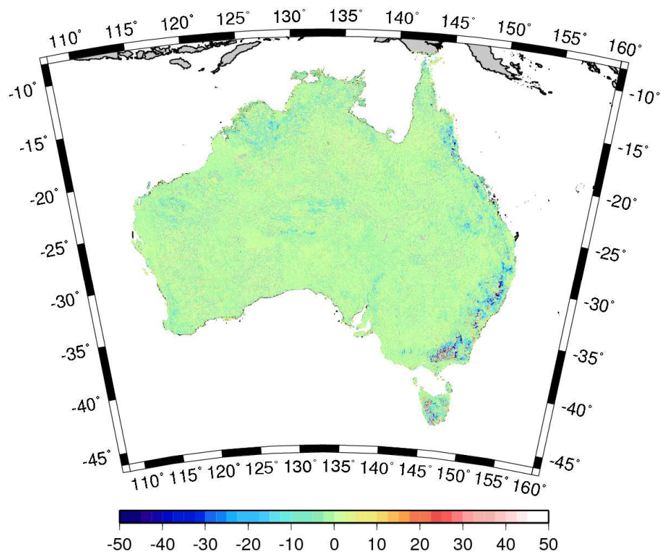
Fig 11. Differences between free-air gravity anomalies from EGM2008 and Australian free-air gravity anomalies on land [Lambert projection; units in mGal].
