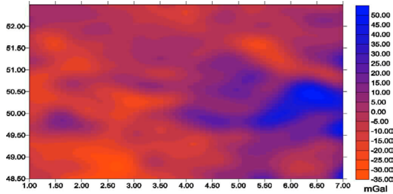
Figure 2c - The GPM98CR gravity anomaly
