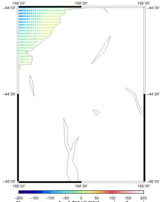
D output: masked DNSC08 marine free-air anomalies (to be used as reinforcement for step E) (units in mGal)
