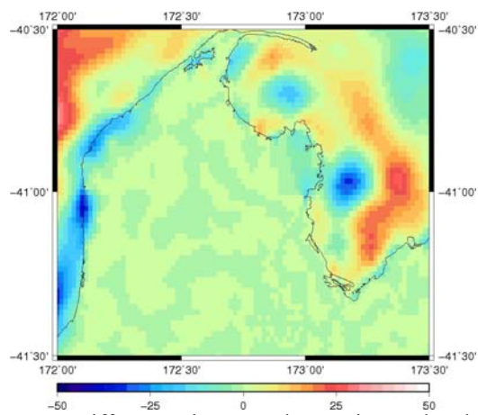
E: Differences between the two interpolated Bouguer anomaly grids
