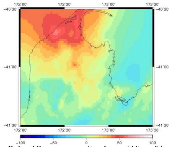
B: Land Bouguer anomalies, from gridding of A using surface
