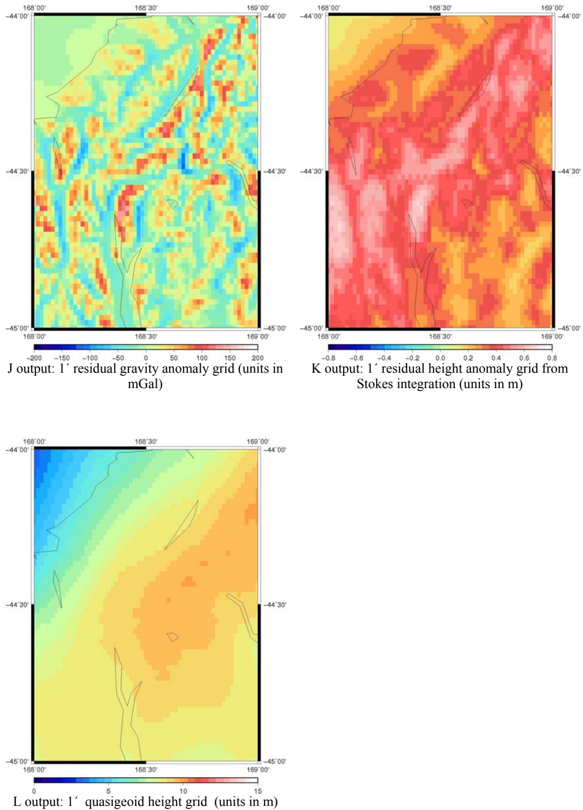
Figure 19. Overview of computation steps A-L for a 1°x1° tile in Northern Fiordland, South Island (Mercator projections)
