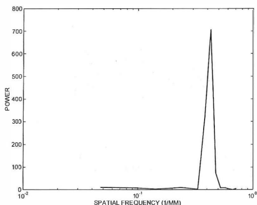
Fig. 9: Power spectrum of NA3000 results at a distance of 19 m and sampling interval of 0.7 mm
