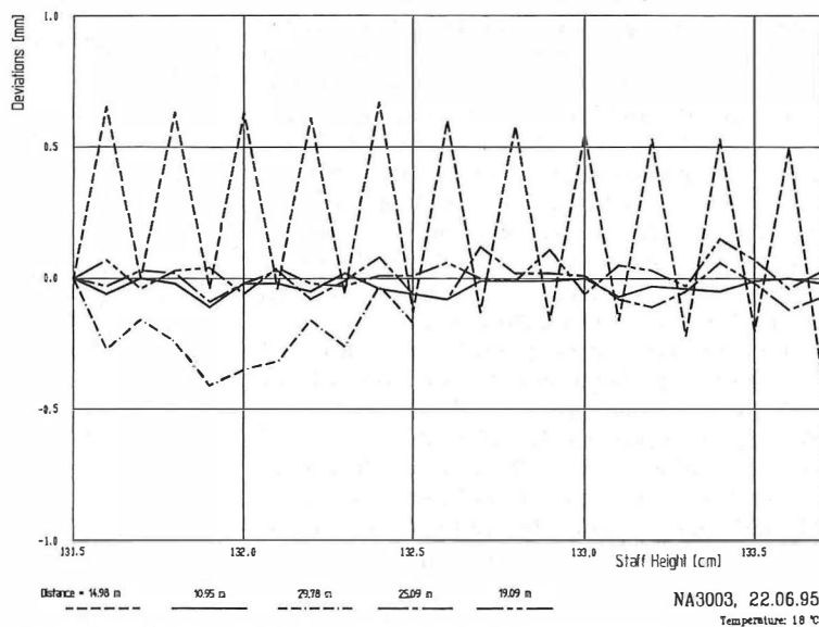
Fig. 11: Results with the NA3003 level in an open air environment
