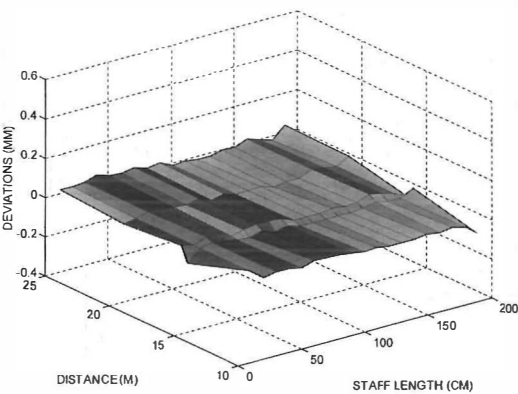
Fig. 4: Deviations of DiNi10 level readings
