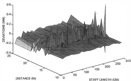
Fig. 6: Deviations of NA3000/3 readings
