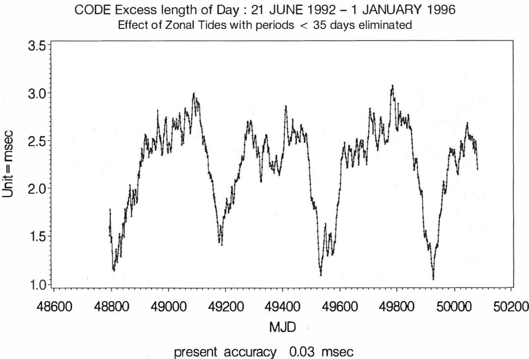
Fig. 3: CODE LoD-estimates after removal of zonal tides
