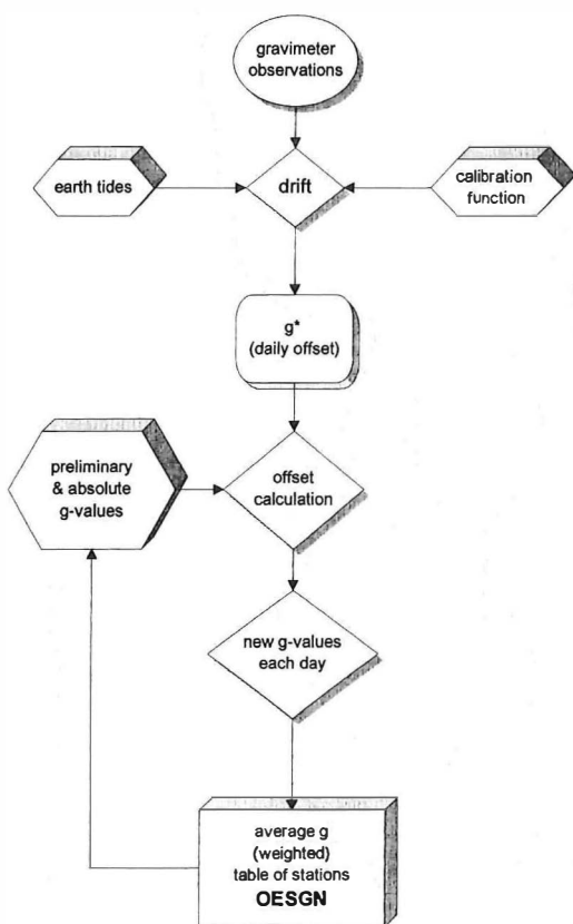
Fig. 3: Data flow diagram of the iterative method
