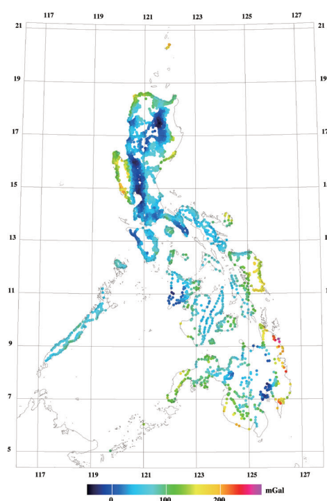
Fig. 7. Distribution of land gravity points used in PGM2018.
