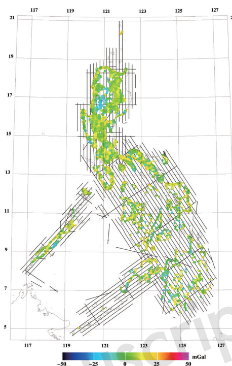
Fig. 8. Differences between airborne and land anomalies for the PGM2018 geoid.
